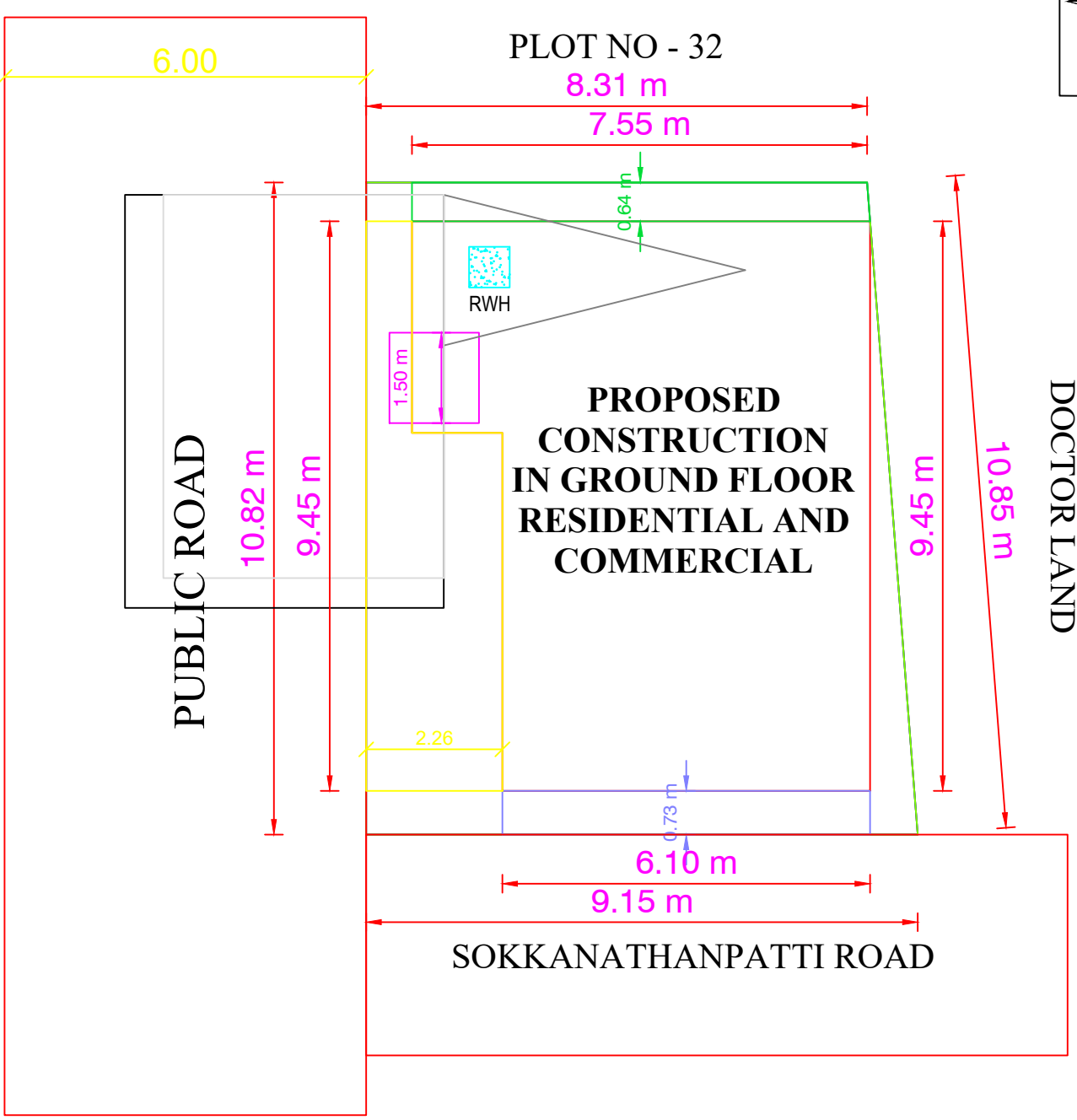
SITE PLAN
