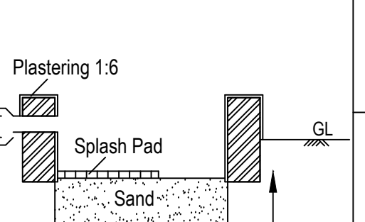
FOUNDATION DETAILS
