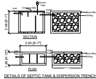
DETAILS OF SEPTIC TANK & DISPERSION TRENCH
