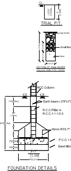
FOUNDATION DETAILS
