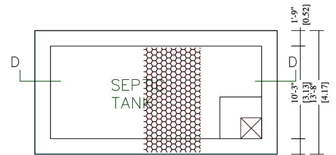
PLAN OF SEPTIC TANK SCALE 1"=2'0"
