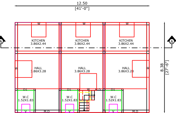
PROPOSED 3NOS.DWELLING RESIDENTIAL GROUND FLOOR
