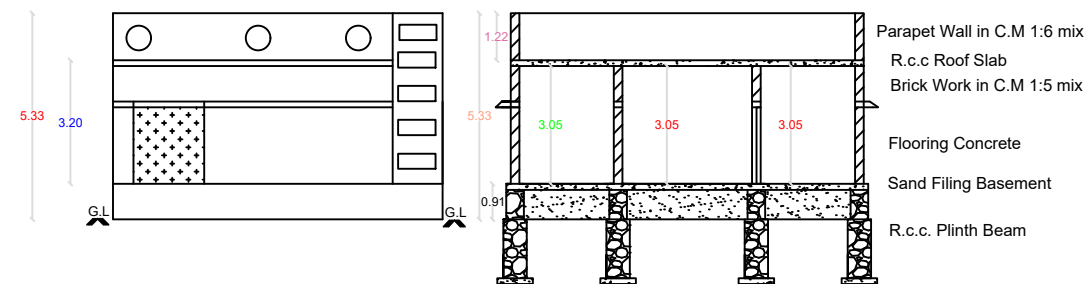
SECTION ON A-A
