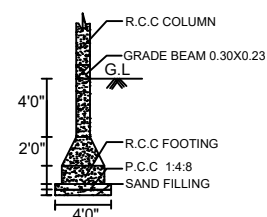
COLOUMN FOUNDATION DETAILS
