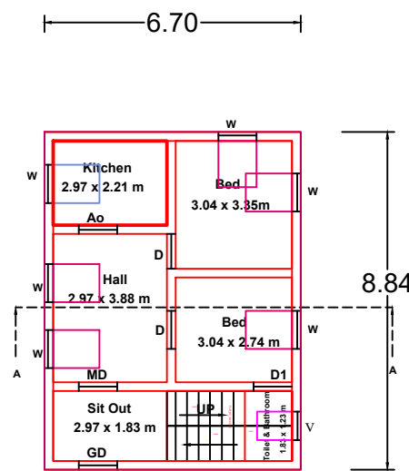
Ground Floor Plan North facing
