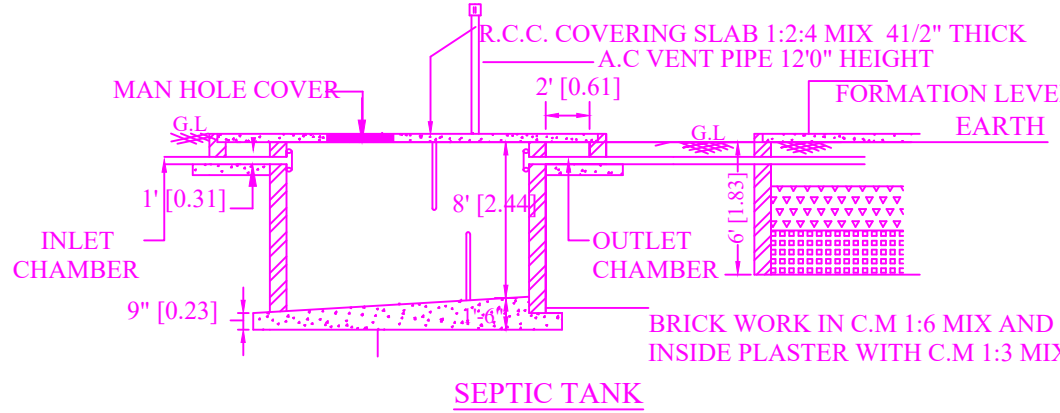
SEPTIC TANK
