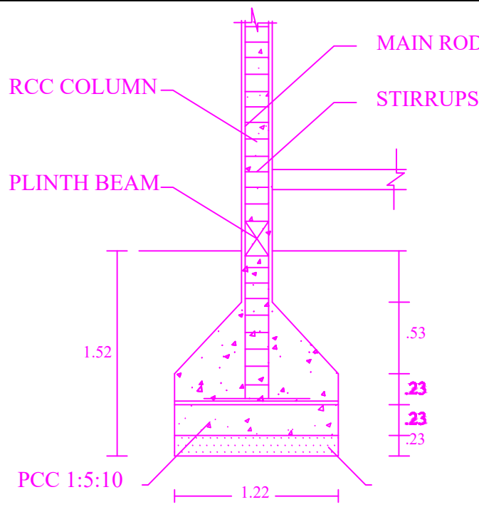
COLUMN DETAILS
