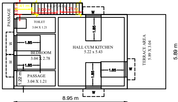
EXISTING GROUND FLOOR AREA
