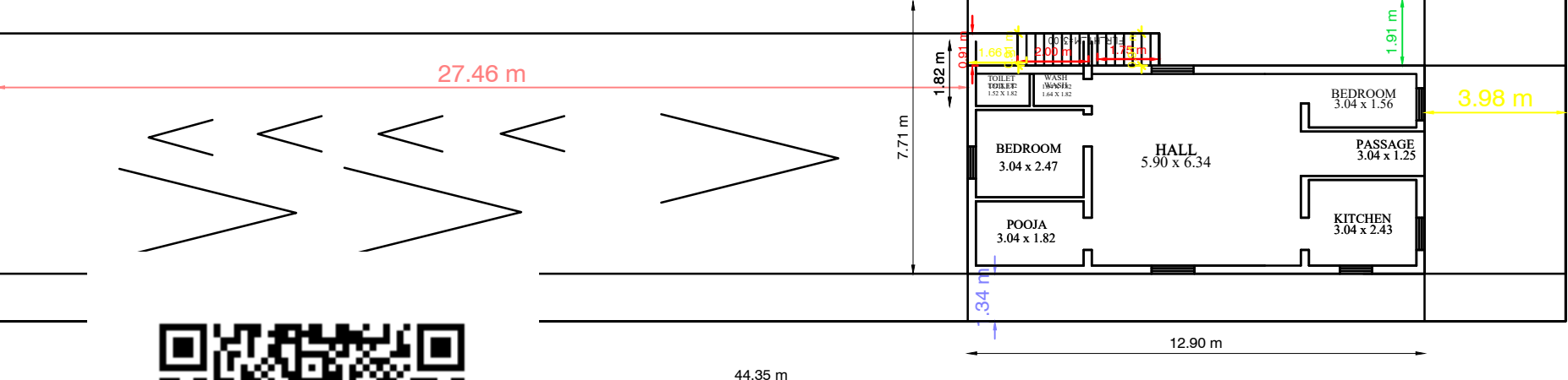
EXISTING GROUND FLOOR AREA
