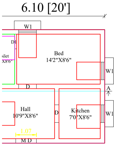
PROPOSED GROUND FLOOR PLAN ROW HOUSE-2
