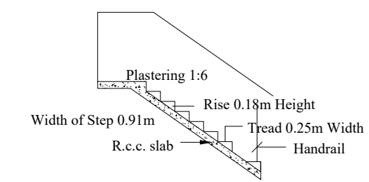
DETAILS OF STAIR CASE
