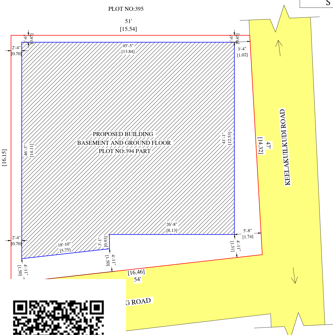
SITE PLAN
