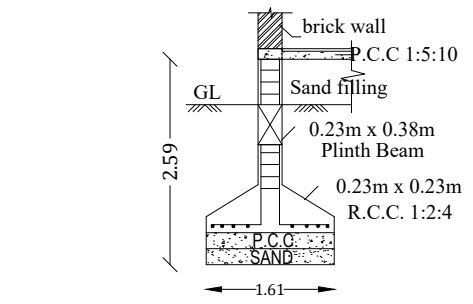
FOUNDATION DETAILS
