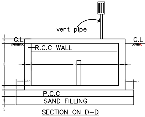
SECTION ON D-D
