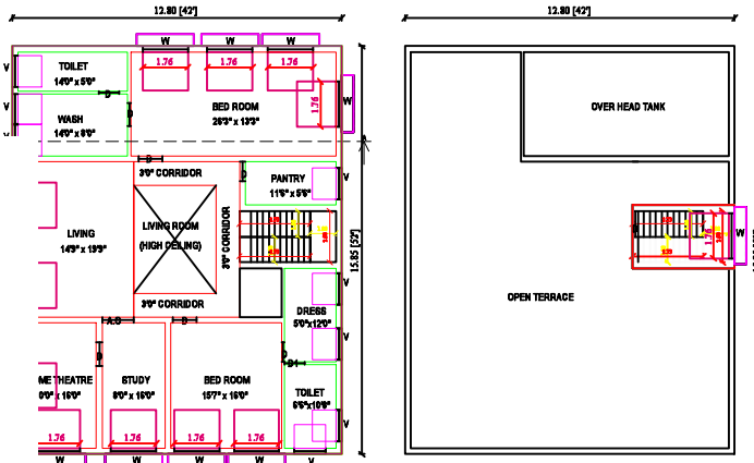
PRO.FIRST FLOOR PLAN
