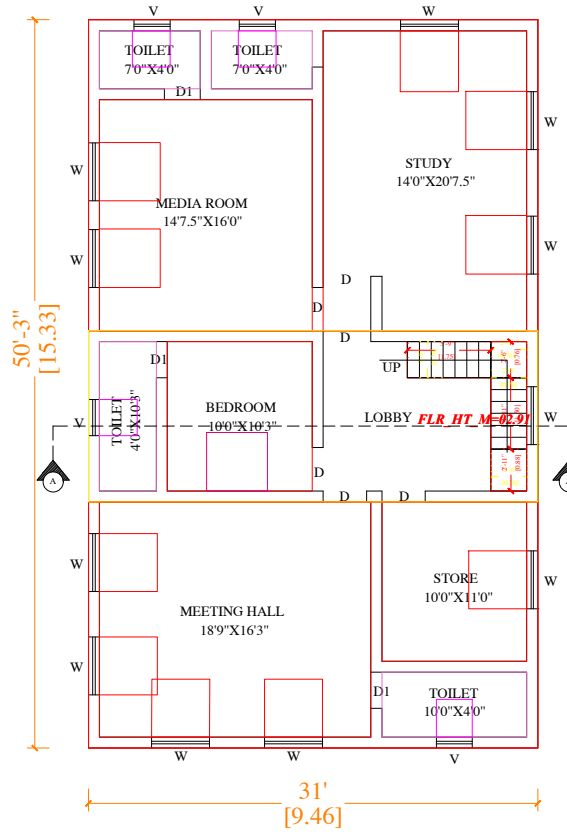
EXISTING & PROPOSED FIRST FLOOR PLAN
