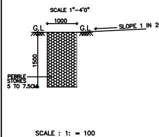
SUMP DETAIL
