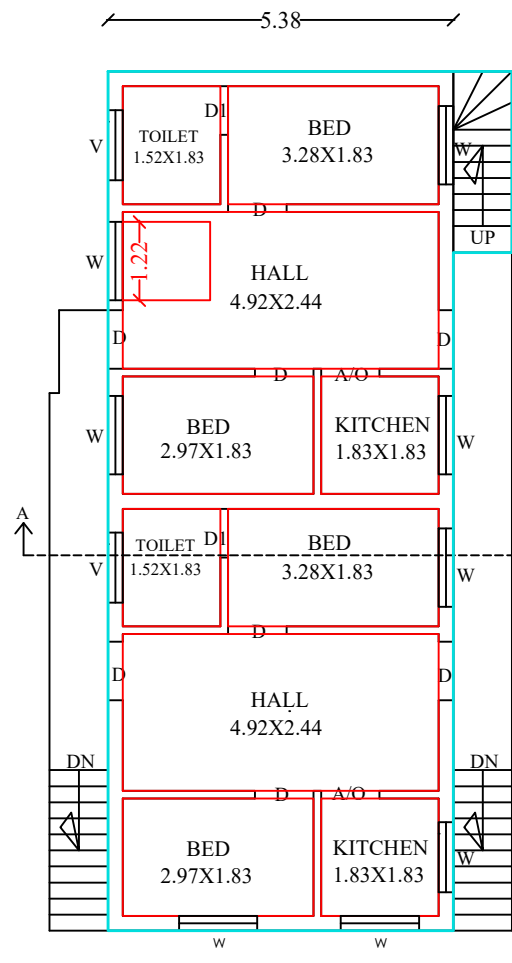
EXG.FIRST FLOOR PLAN
