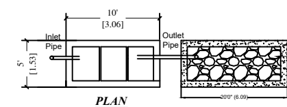
DETAILS OF SEPTIC TANK & DISPERSION TRENCH
