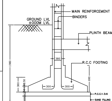
TYPICAL SECTION OF R.C.C COLUMN FOUNDATION SCALE : 1" = 2'-0"
