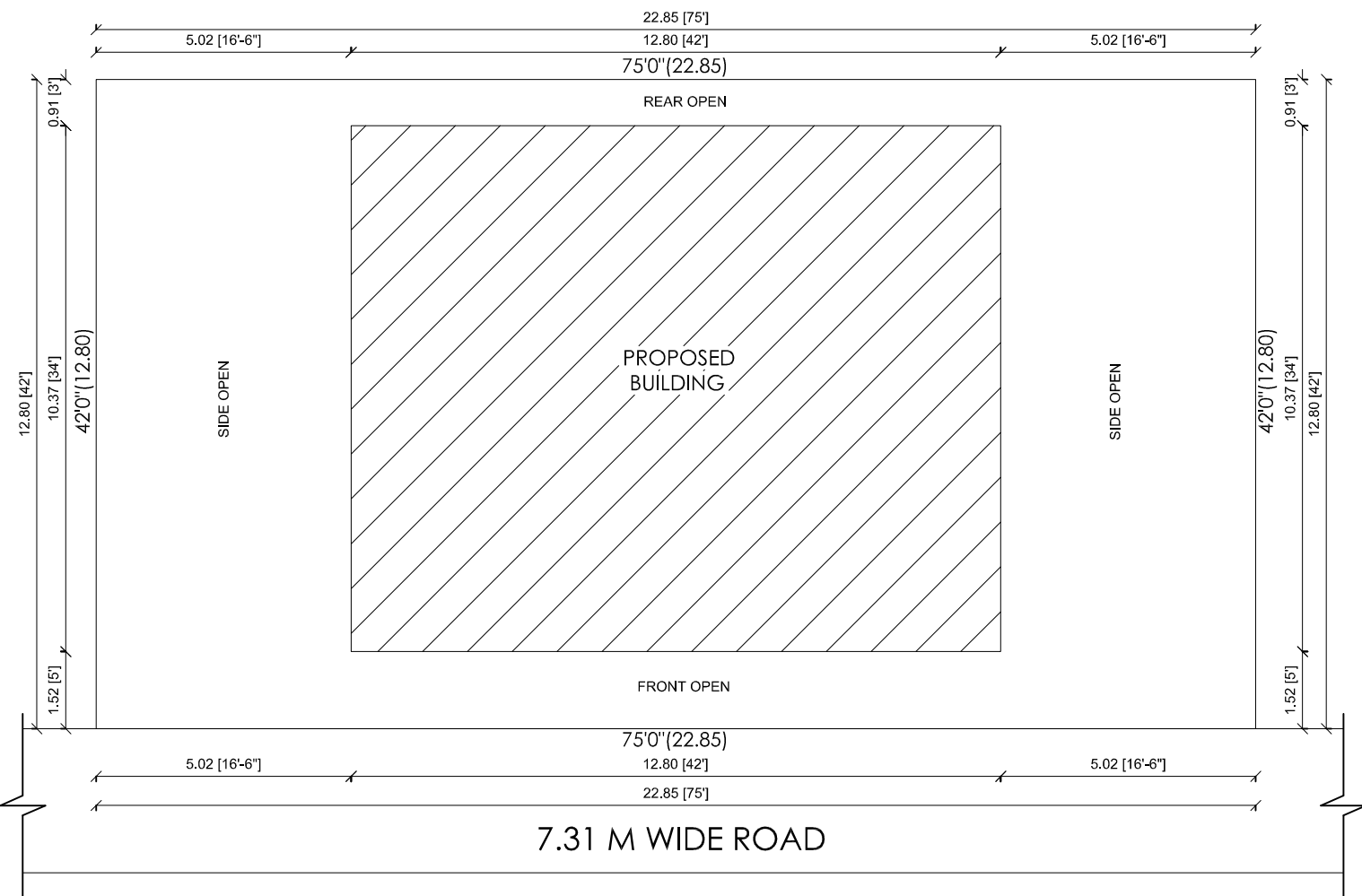
SITE PLAN
