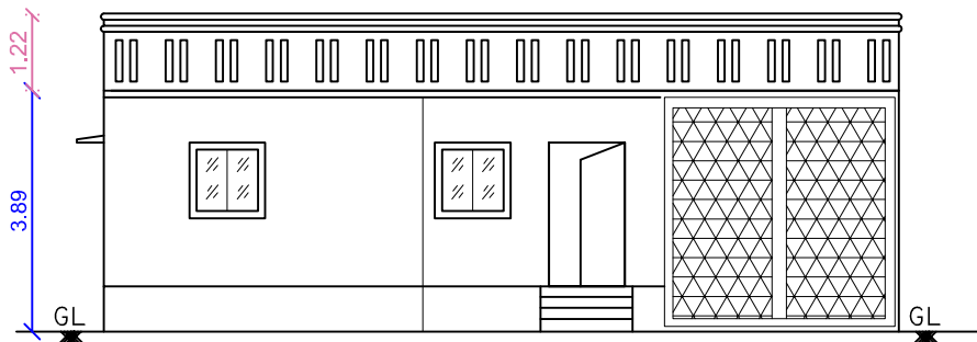
FRONT ELEVATION
