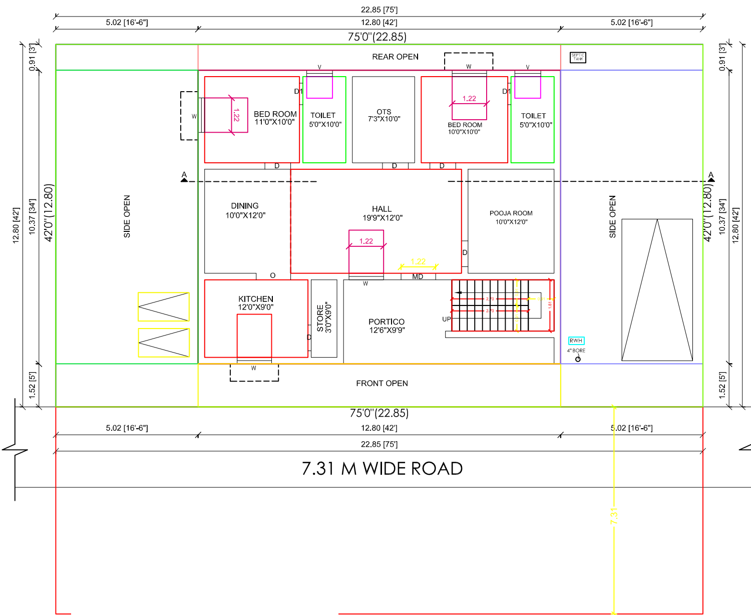
ROUND FLOOR PLAN
