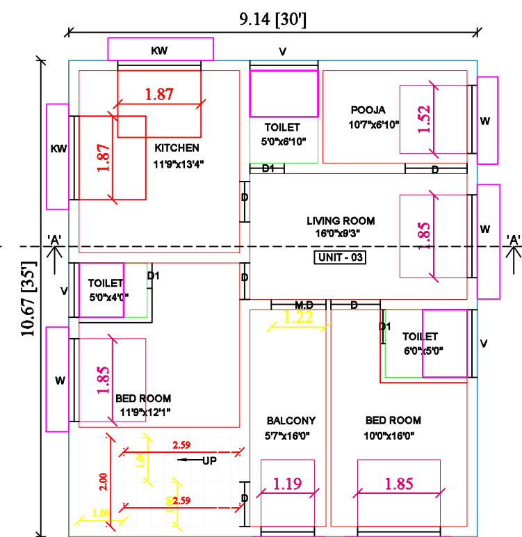
PRO.SECOND FLOOR PLAN
