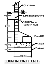
FOUNDATION DETAILS
