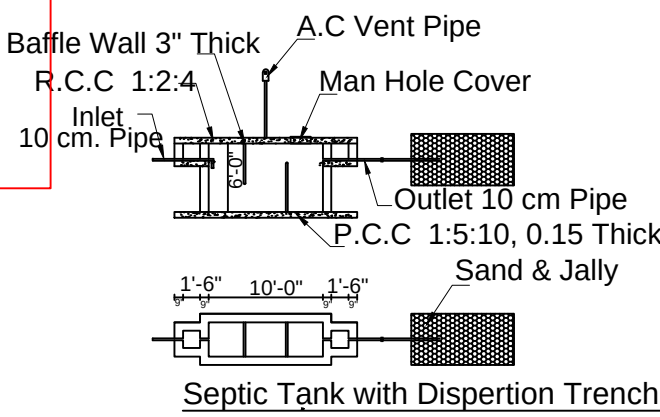
Septic Tank with Dispersion Trench
