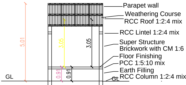
SECTION ON "VR"
