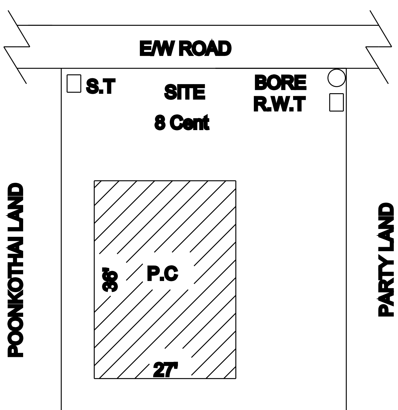
KEY PLAN
