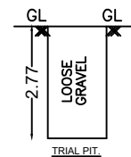
TRIAL PIT
