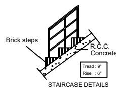
STAIRCASE DETAILS
