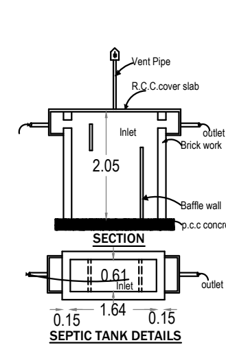
SEPTIC TANK DETAILS
