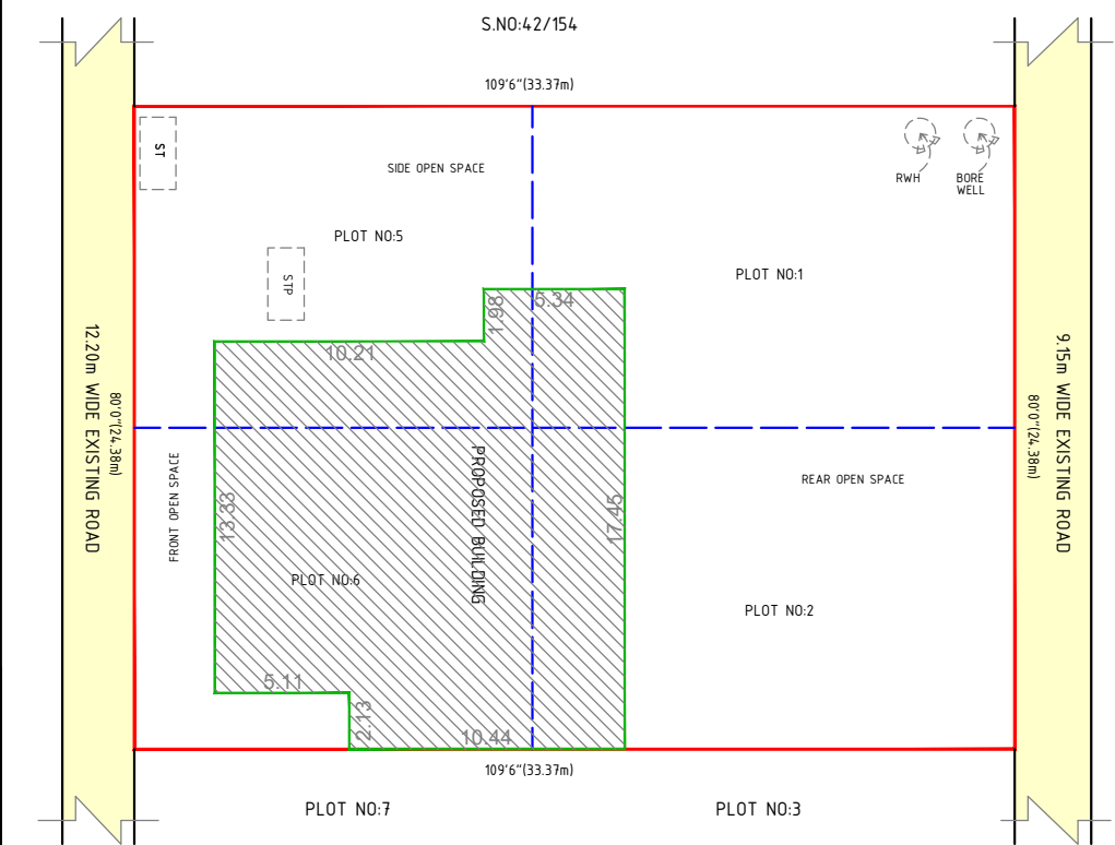
TOPO PLAN
