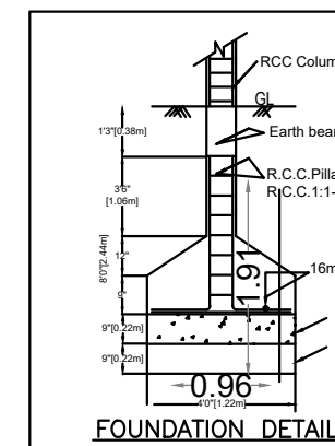
FOUNDATION DETAILS
