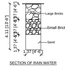
SECTION OF RAIN WATER
