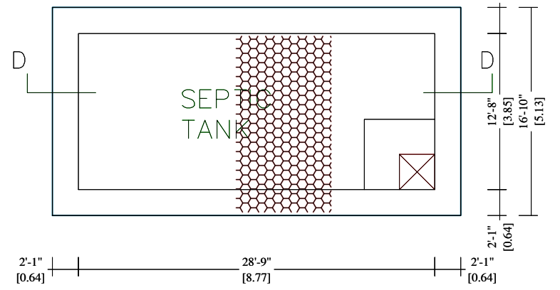
PLAN OF SEPTIC TANK SCALE 1"=2'0"
