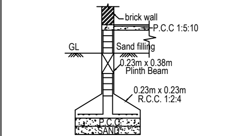
FOUNDATION DETAILS
