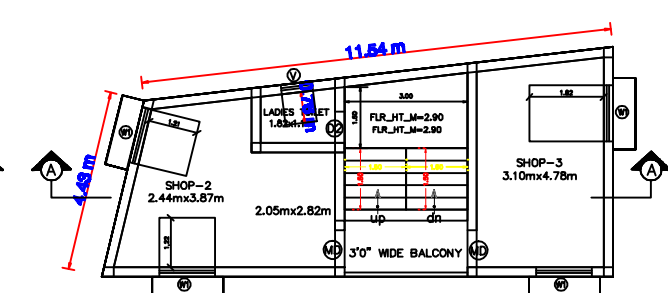
PROPOSED FIRST FLOOR PLAN
