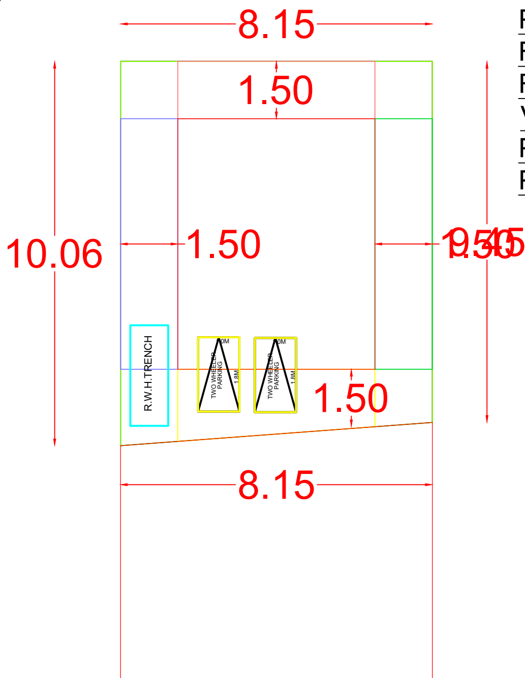
SITE PLAN
