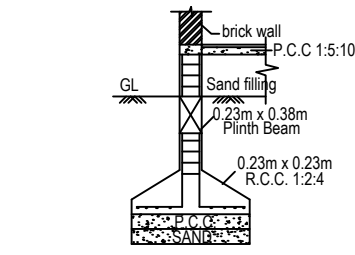
FOUNDATION DETAILS
