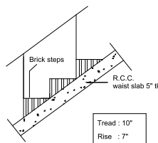
STAIRCASE DETAILS-nts
