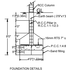
FOUNDATION DETAILS
