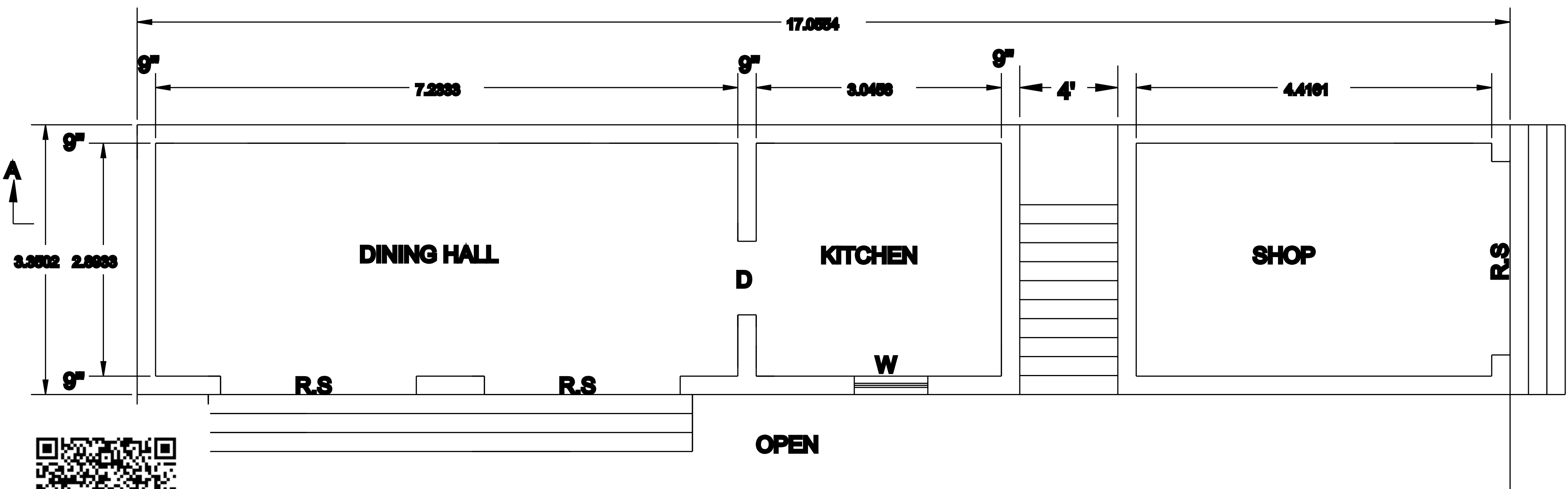
PROSED G.F PLAN
