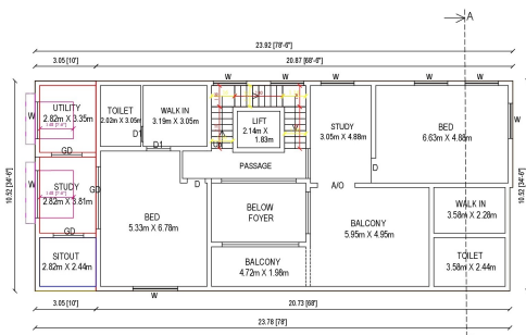
EXISTING & PROPOSED FIRST FLOOR PLAN
