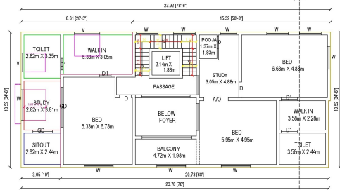
EXISTING & PROPOSED SECOND FLOOR PLAN
