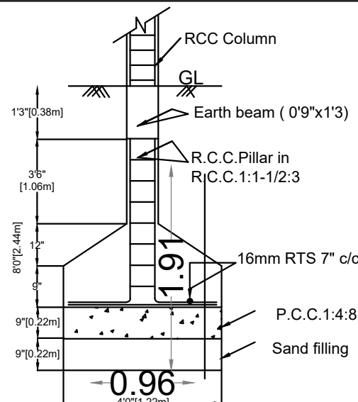
FOUNDATION DETAILS
