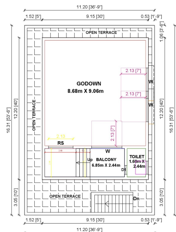
PRO-NON-RES SECOND FLOOR PLAN
