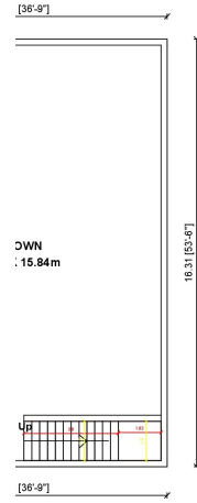
IRST FLOOR PLAN
