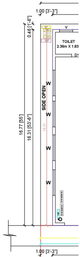
EXI - NON-RES GROUND FLOOR PLAN
