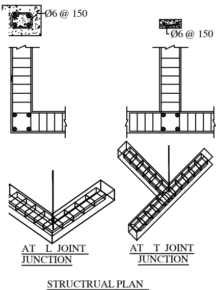
STRUCTURAL PLAN
