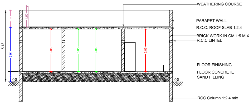
SECTION - 'IR'
