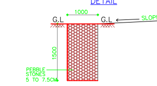
SECTION OF PEBBLE TRENCH
