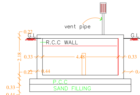
SECTION ON D-D
