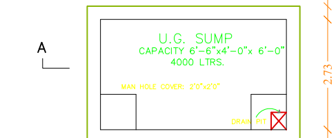
SUMP DETAIL SCALE 1"=4'0"
