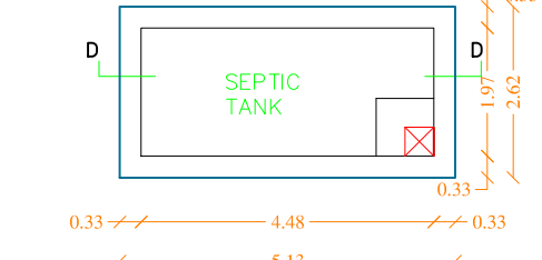
PLAN OF SEPTIC TANK SCALE 1"=2'0"
