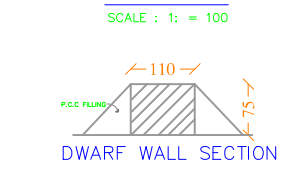
DWARF WALL SECTION NOT TO SCALE
