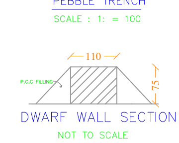
DWARF WALL SECTION NOT TO SCALE
