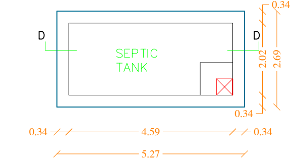
PLAN OF SEPTIC TANK SCALE 1"-2'0"
