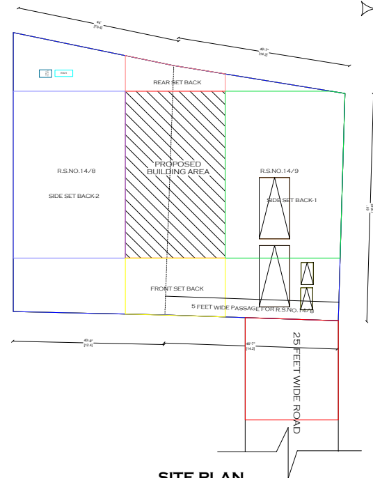
SITE PLAN
