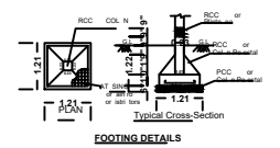
Typical Cross-Section
