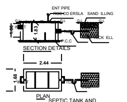
SECTION DETAILS
