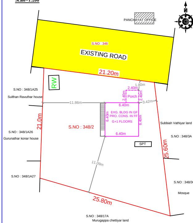
TOPO PLAN Not to scale
