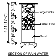
SECTION OF RAIN WATER
