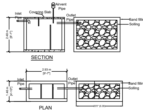
Details of solar water heating system
