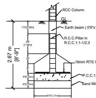
FOUNDATION DETAILS
