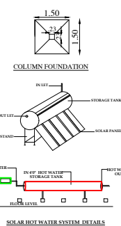
SOLAR HOT WATER SYSTEM DETAILS
