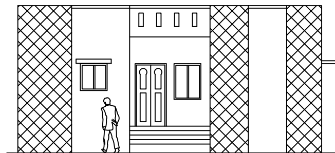
FRONT ELEVATION.
