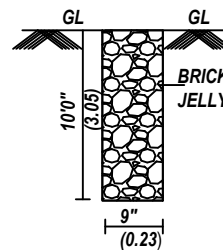
PERCULATION PIT
