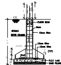
FOUNDATION DETAILS
