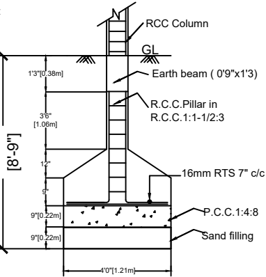
FOUNDATION DETAILS
