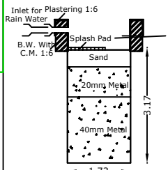
RAIN WATER PERCOLATION P
