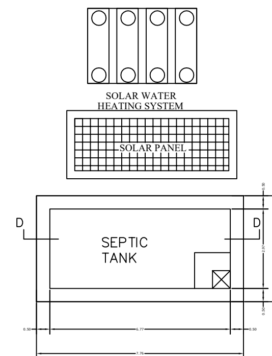
PLAN OF SEPTIC TANK SCALE 1"=2'0"
